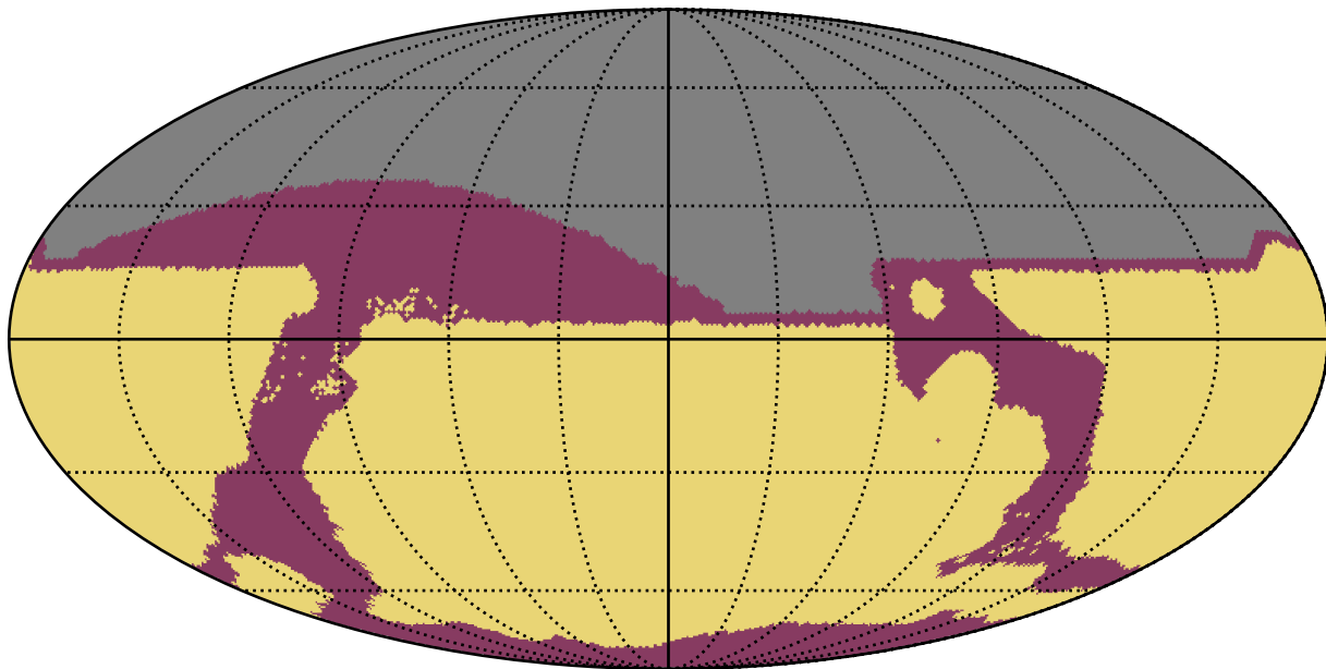
noroll_mjdp0_v3.4_10yrs All sky: RapidRevisits
