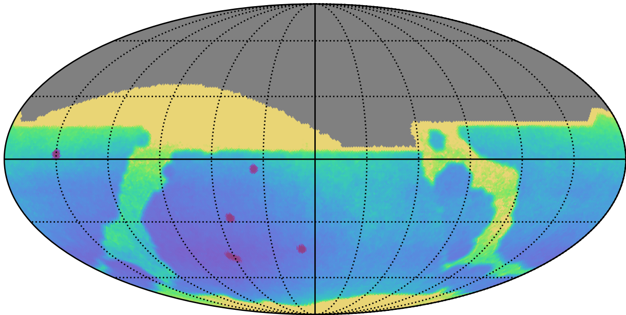
noroll_mjdp0_v3.4_10yrs All sky: Parallax Uncert @ 22.4
