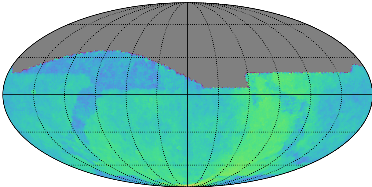
noroll_mjdp0_v3.4_10yrs All sky: Parallax Coverage @ 24.0
