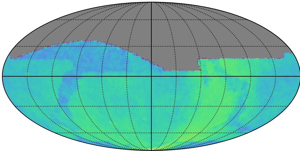
noroll_mjdp0_v3.4_10yrs All sky: Parallax Coverage @ 22.4
