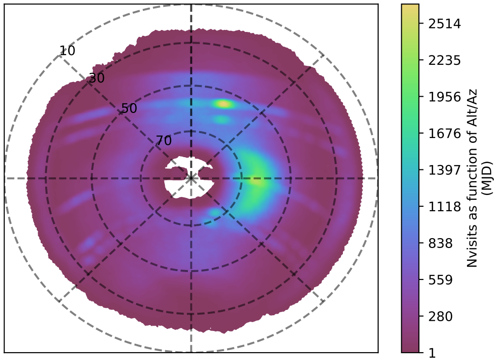
noroll_mjdp0_v3.4_10yrs z band: Nvisits as function of Alt/Az
