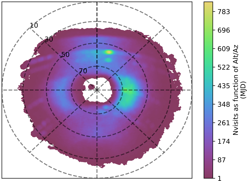
noroll_mjdp0_v3.4_10yrs u band: Nvisits as function of Alt/Az
