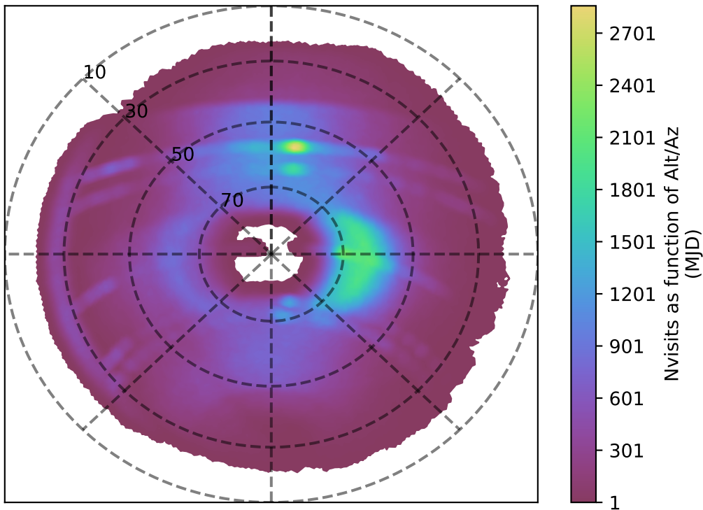
noroll_mjdp0_v3.4_10yrs r band: Nvisits as function of Alt/Az
