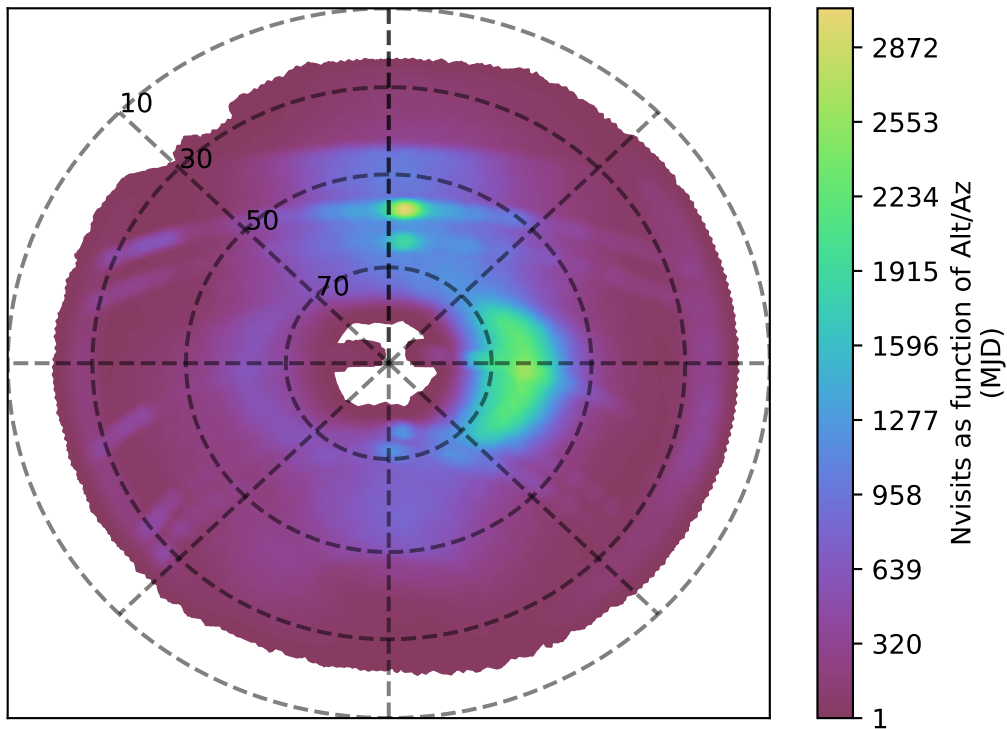
noroll_mjdp0_v3.4_10yrs i band: Nvisits as function of Alt/Az
