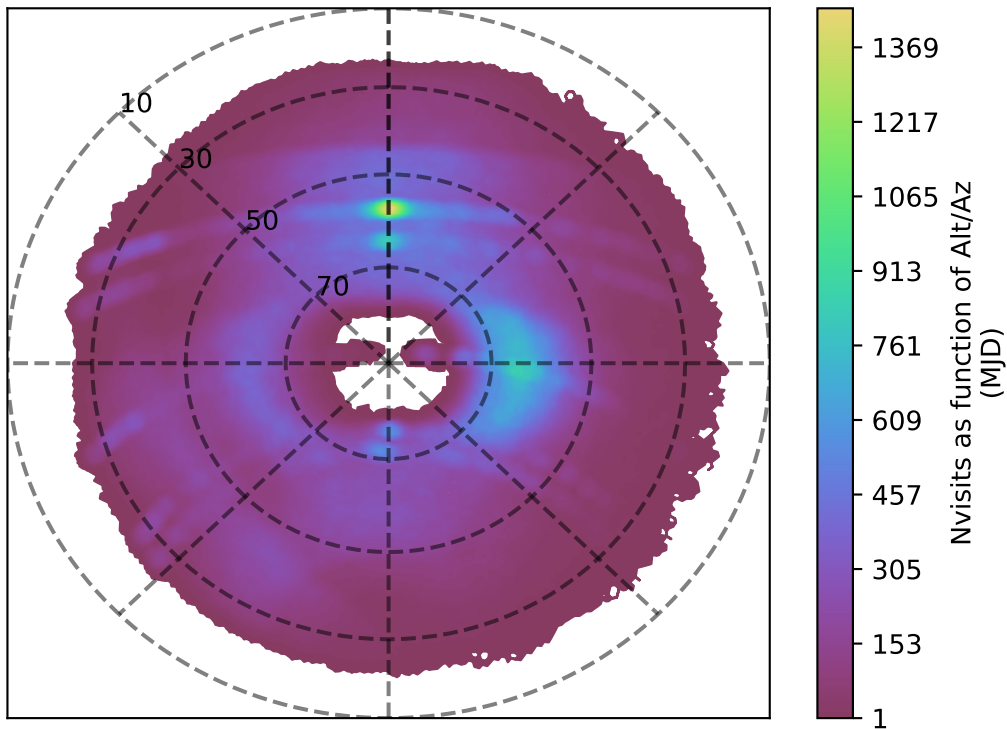
noroll_mjdp0_v3.4_10yrs g band: Nvisits as function of Alt/Az
