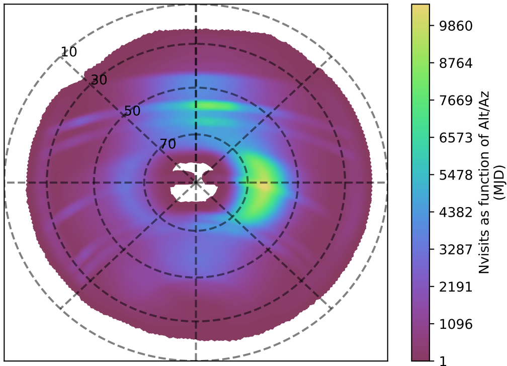
noroll_mjdp0_v3.4_10yrs all bands: Nvisits as function of Alt/Az
