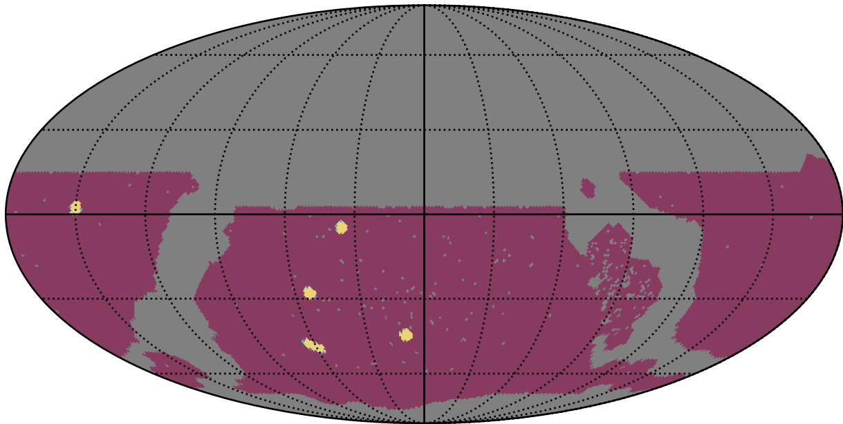
noroll_mjdp0_v3.4_10yrs WFD: NumberOfQuickRevisits
