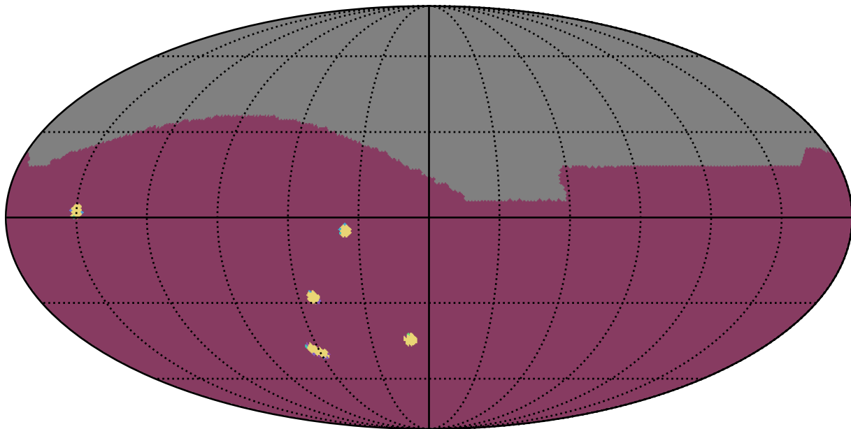
noroll_mjdp0_v3.4_10yrs All sky: NumberOfQuickRevisits
