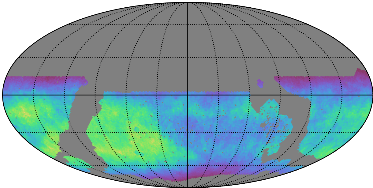
noroll_mjdp0_v3.4_10yrs WFD z band: Normalized Teff
