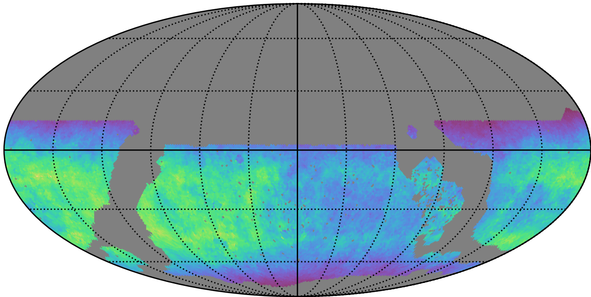
noroll_mjdp0_v3.4_10yrs WFD u band: Normalized Teff
