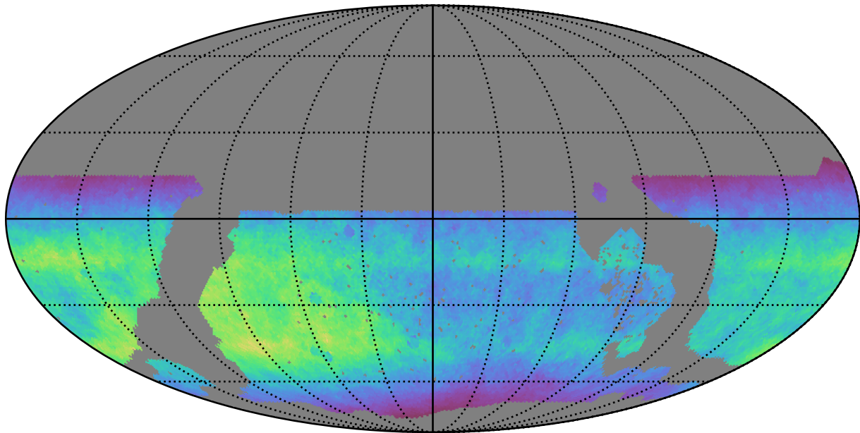
noroll_mjdp0_v3.4_10yrs WFD i band: Normalized Teff
