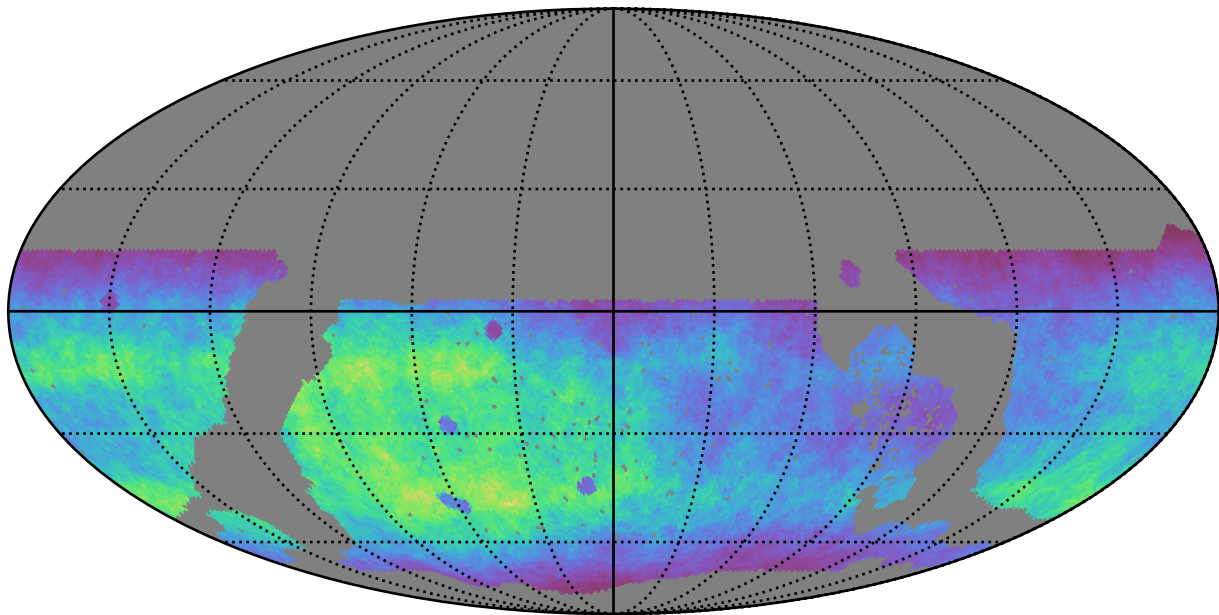
noroll_mjdp0_v3.4_10yrs WFD g band: Normalized Teff
