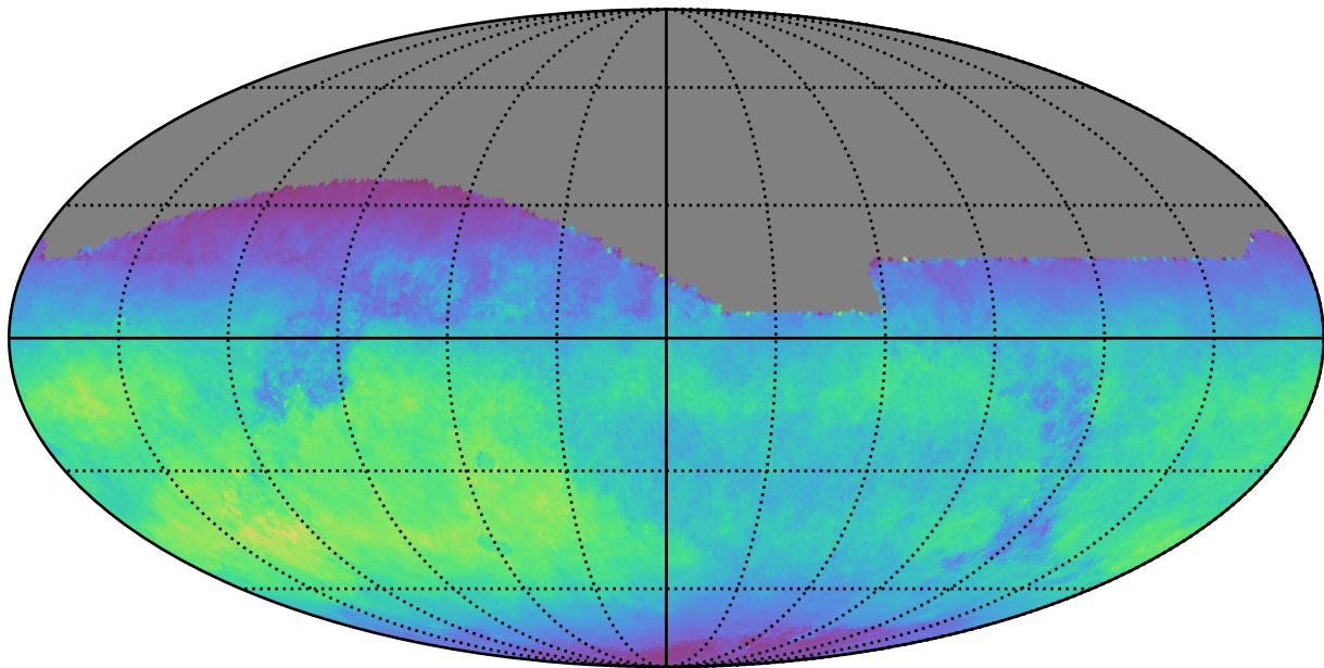
noroll_mjdp0_v3.4_10yrs All sky z band: Normalized Teff
