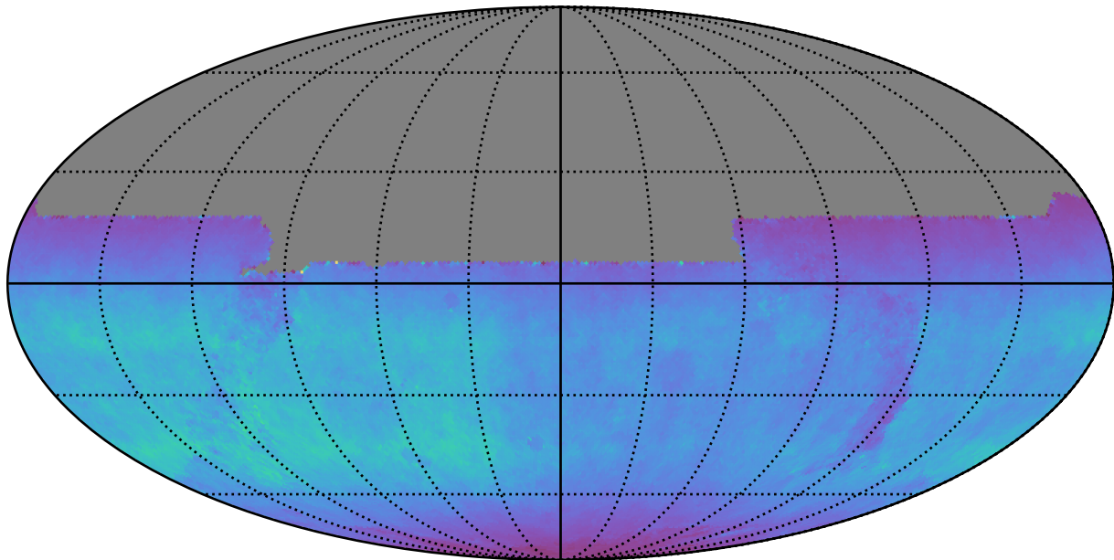
noroll_mjdp0_v3.4_10yrs All sky y band: Normalized Teff
