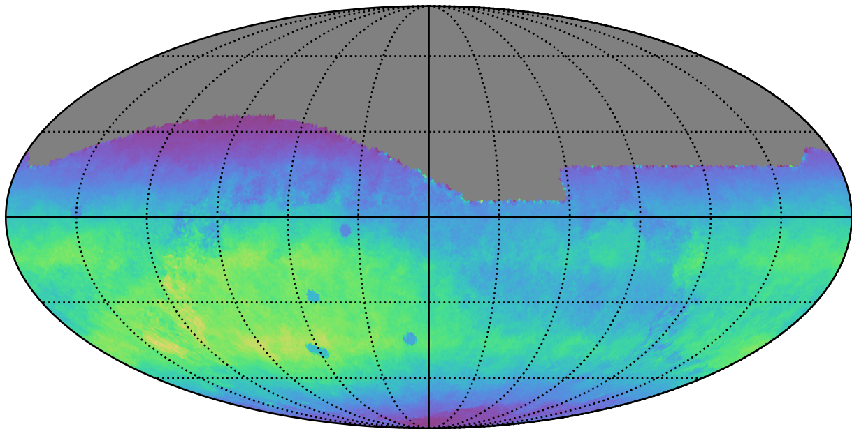
noroll_mjdp0_v3.4_10yrs All sky r band: Normalized Teff
