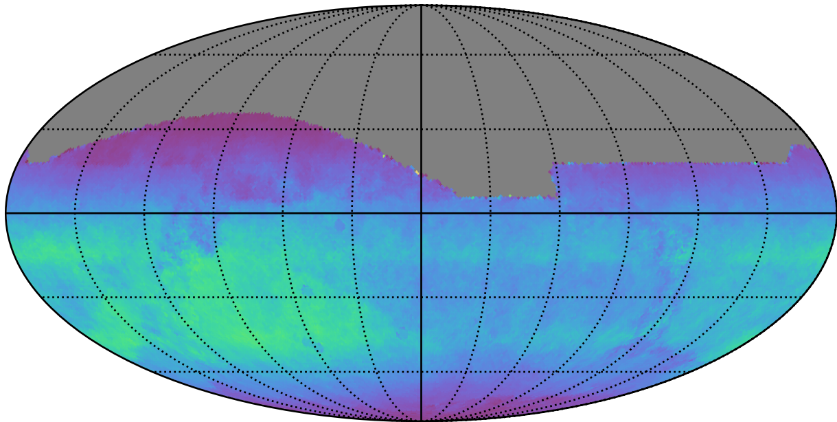
noroll_mjdp0_v3.4_10yrs All sky i band: Normalized Teff
