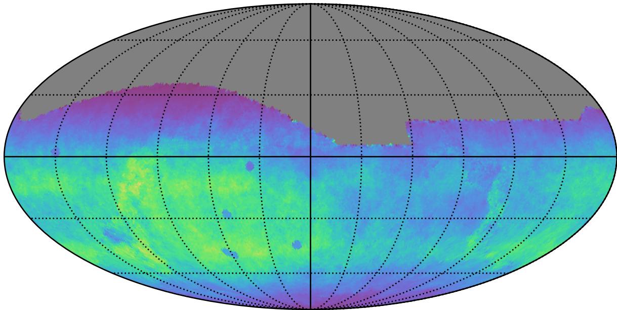
noroll_mjdp0_v3.4_10yrs All sky g band: Normalized Teff
