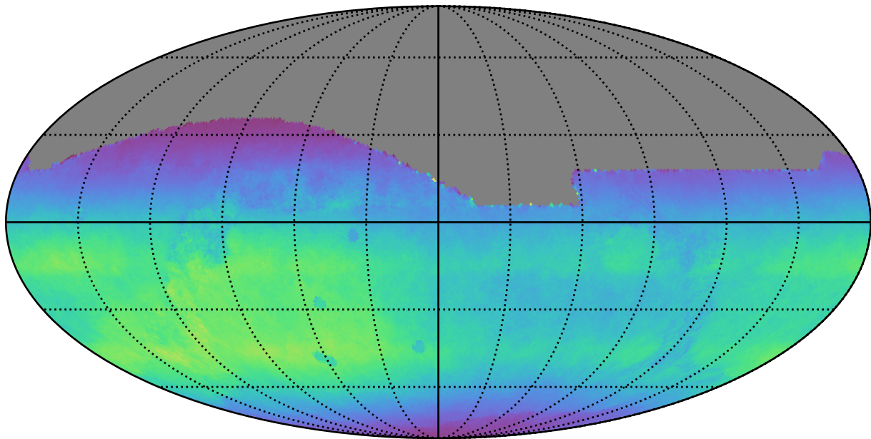
noroll_mjdp0_v3.4_10yrs All sky all bands: Normalized Teff
