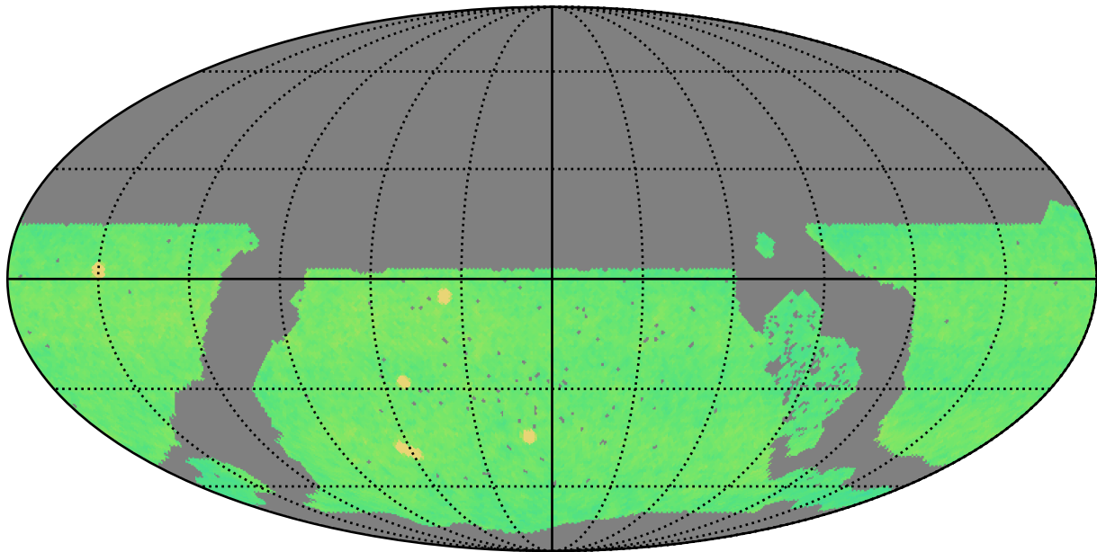
noroll_mjdp0_v3.4_10yrs WFD all bands: N Unique Nights
