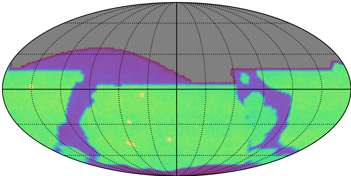
noroll_mjdp0_v3.4_10yrs All sky all bands: N Unique Nights
