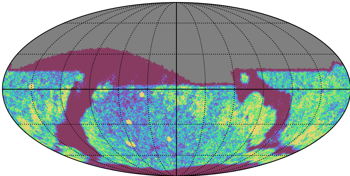
noroll_mjdp0_v3.4_10yrs Yr 1 r band: NVisits
