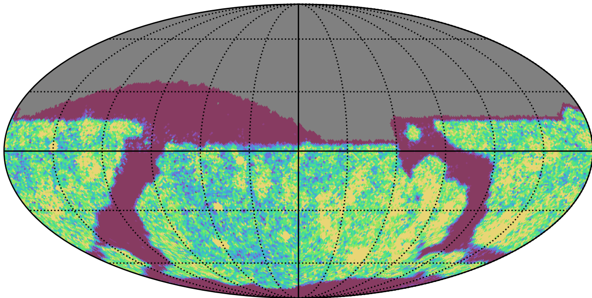
noroll_mjdp0_v3.4_10yrs Yr 1 i band: NVisits
