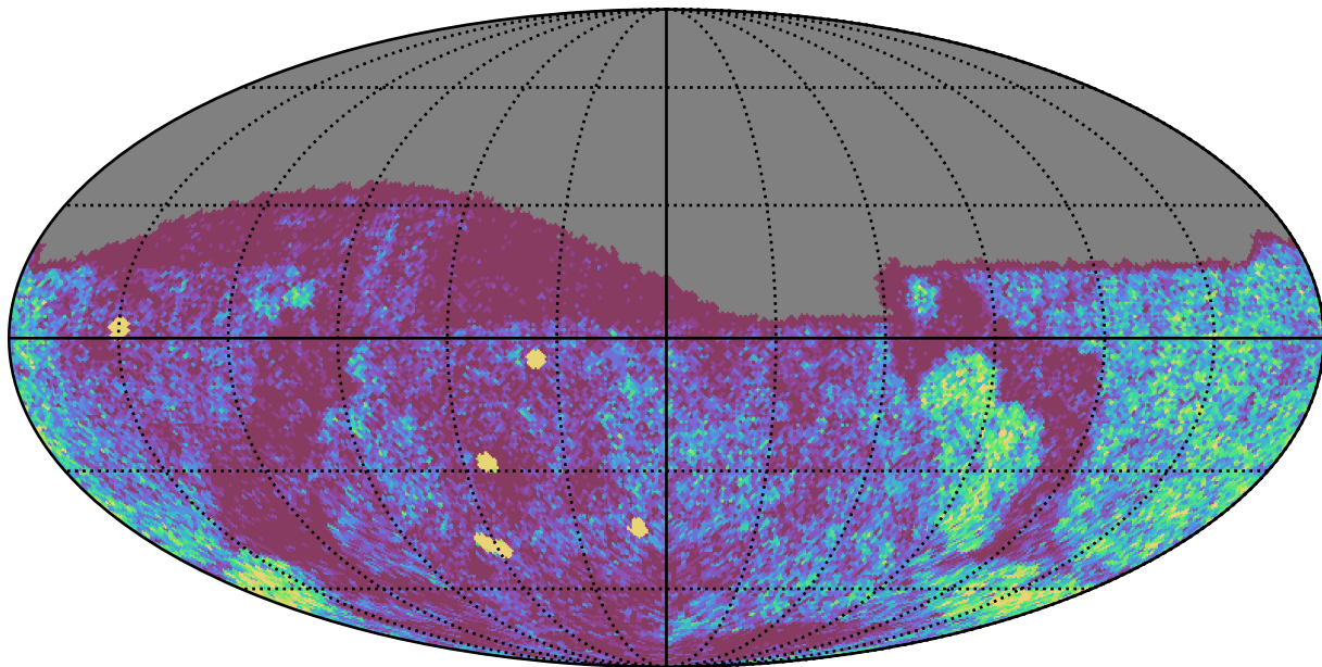
noroll_mjdp0_v3.4_10yrs Yr 1 g band: NVisits
