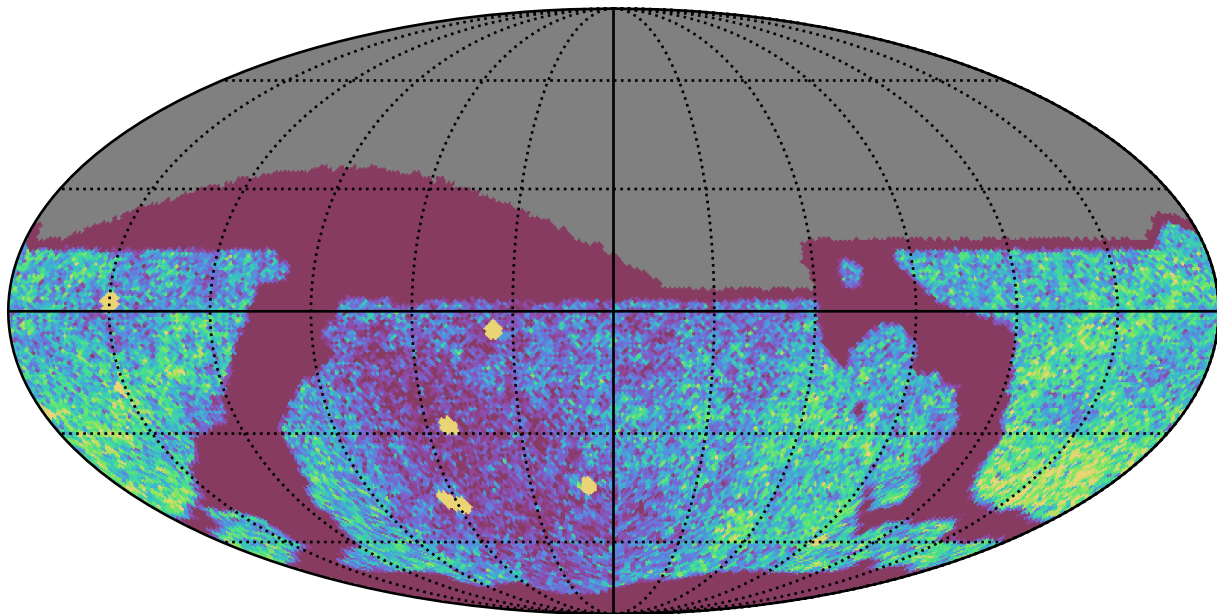
noroll_mjdp0_v3.4_10yrs Yr 1 all bands: NVisits
