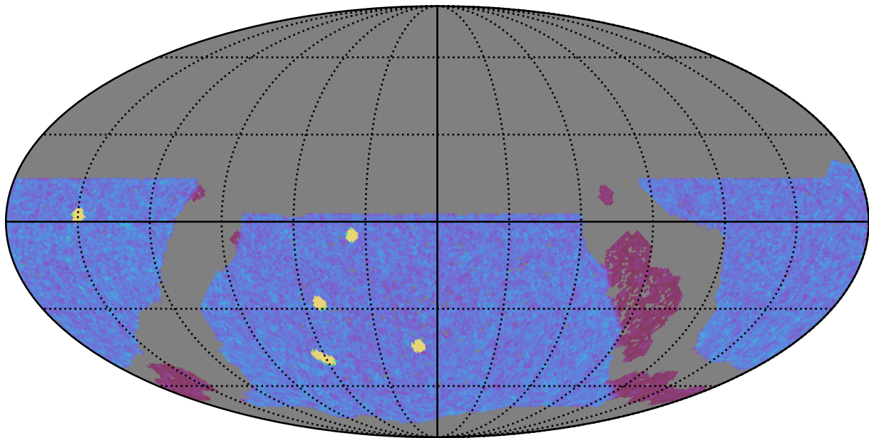
noroll_mjdp0_v3.4_10yrs WFD y band: NVisits
