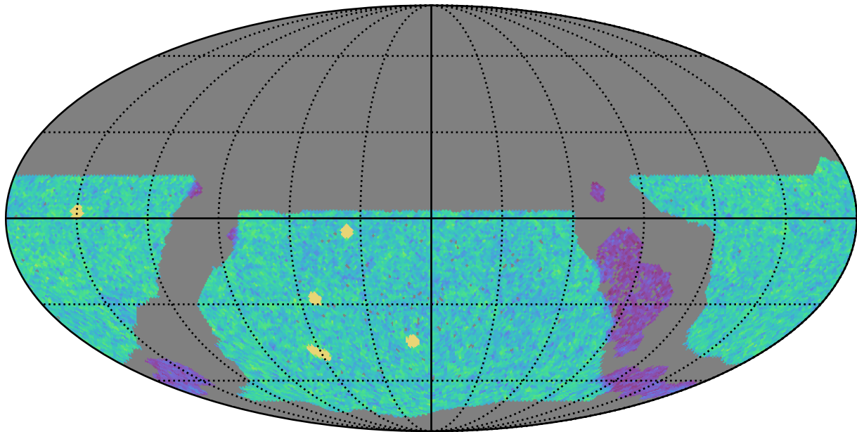
noroll_mjdp0_v3.4_10yrs WFD u band: NVisits
