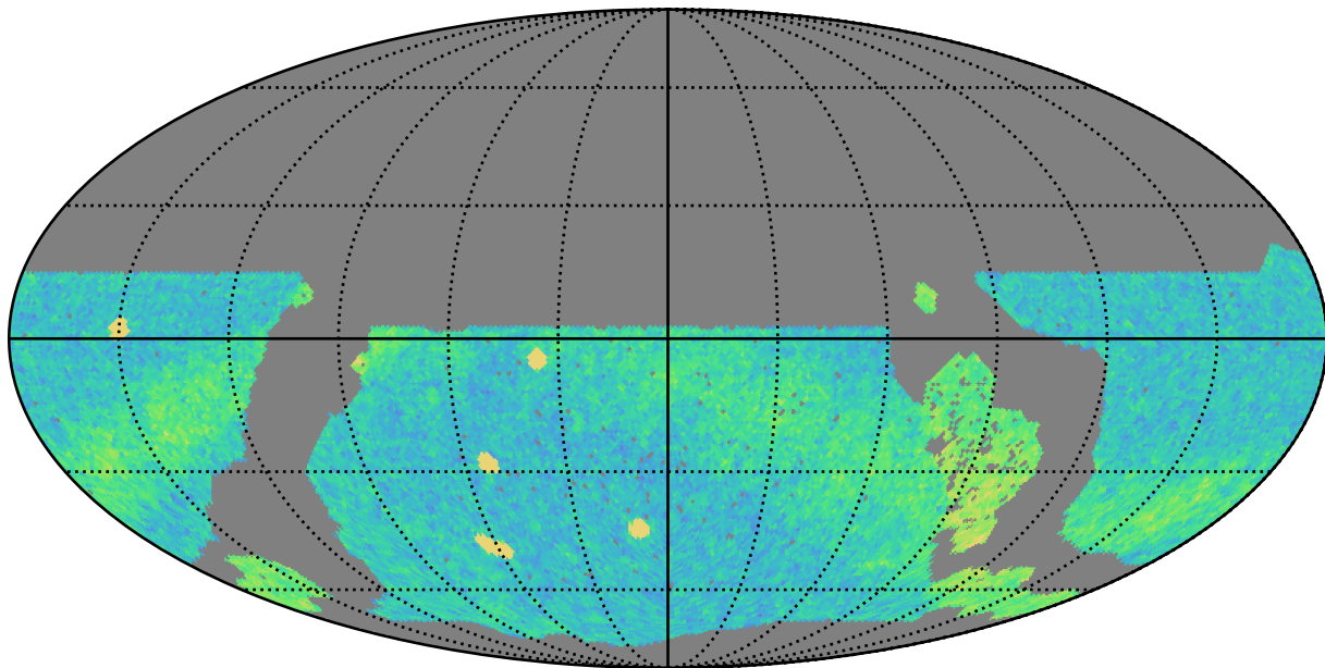
noroll_mjdp0_v3.4_10yrs WFD r band: NVisits
