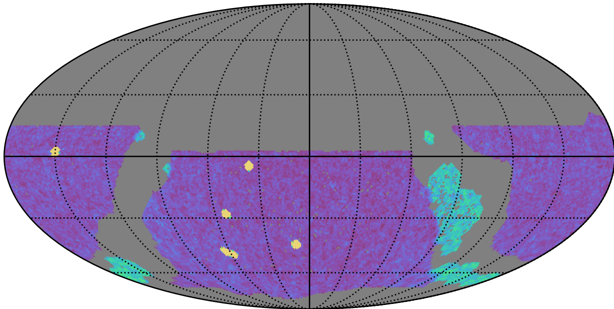
noroll_mjdp0_v3.4_10yrs WFD g band: NVisits
