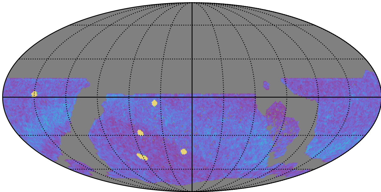
noroll_mjdp0_v3.4_10yrs WFD all bands: NVisits
