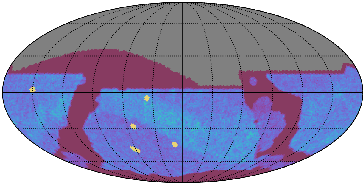
noroll_mjdp0_v3.4_10yrs All sky z band: NVisits
