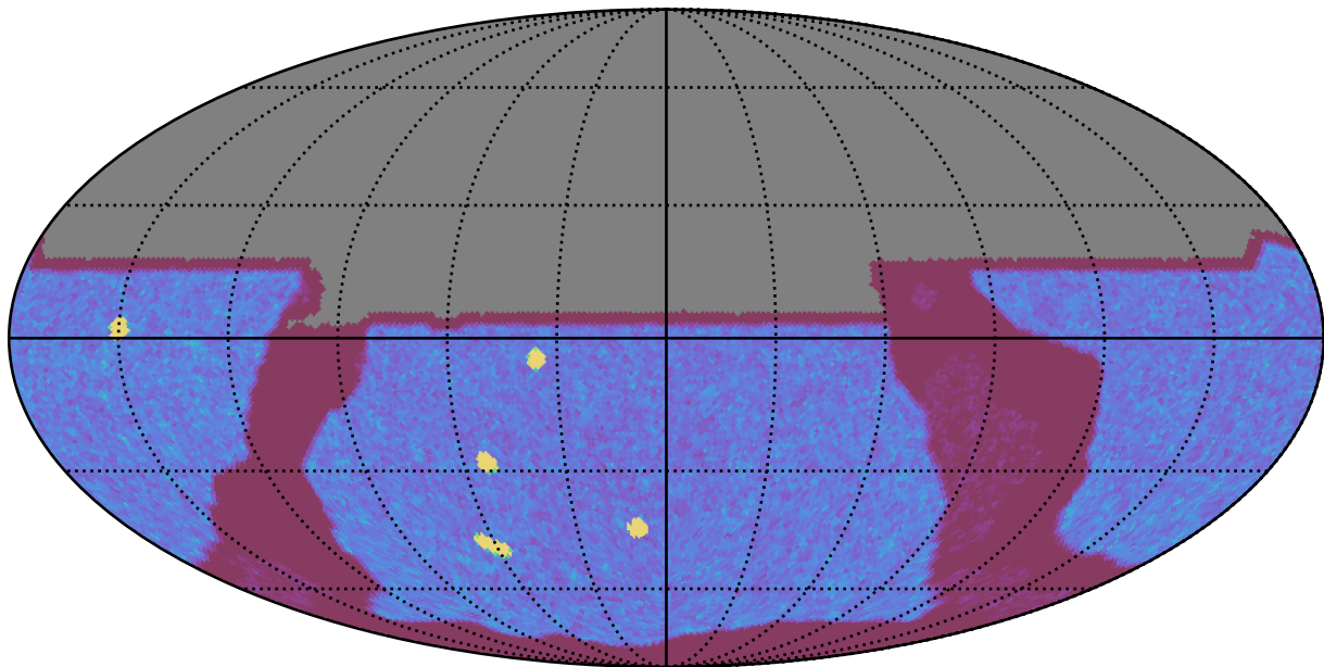
noroll_mjdp0_v3.4_10yrs All sky y band: NVisits
