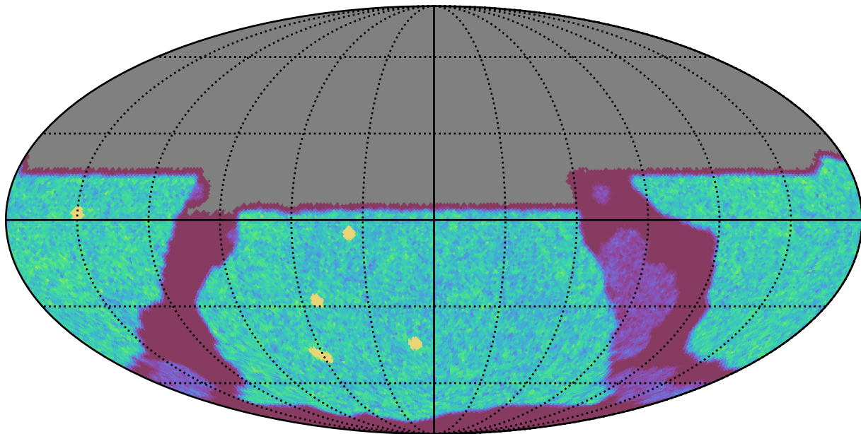
noroll_mjdp0_v3.4_10yrs All sky u band: NVisits
