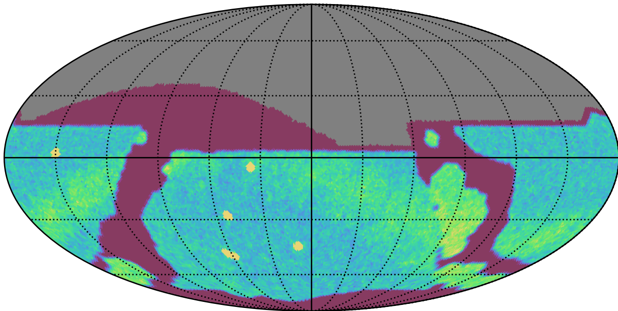
noroll_mjdp0_v3.4_10yrs All sky r band: NVisits
