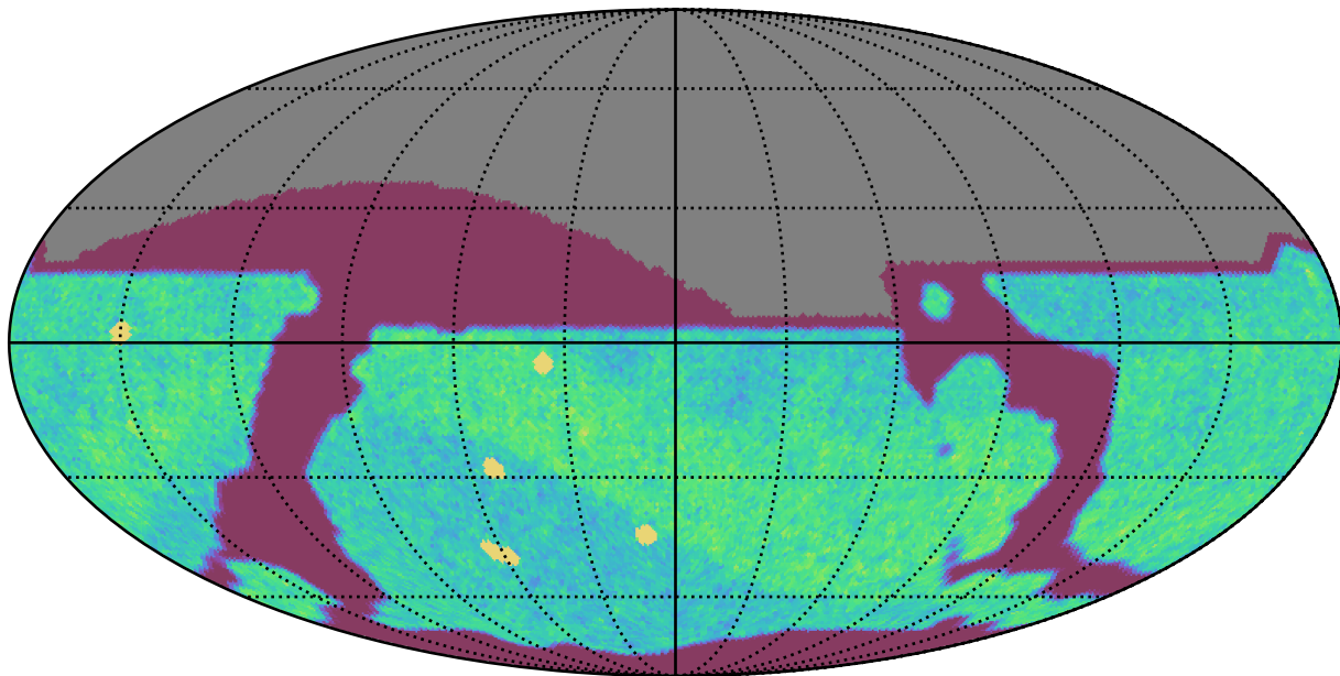
noroll_mjdp0_v3.4_10yrs All sky i band: NVisits
