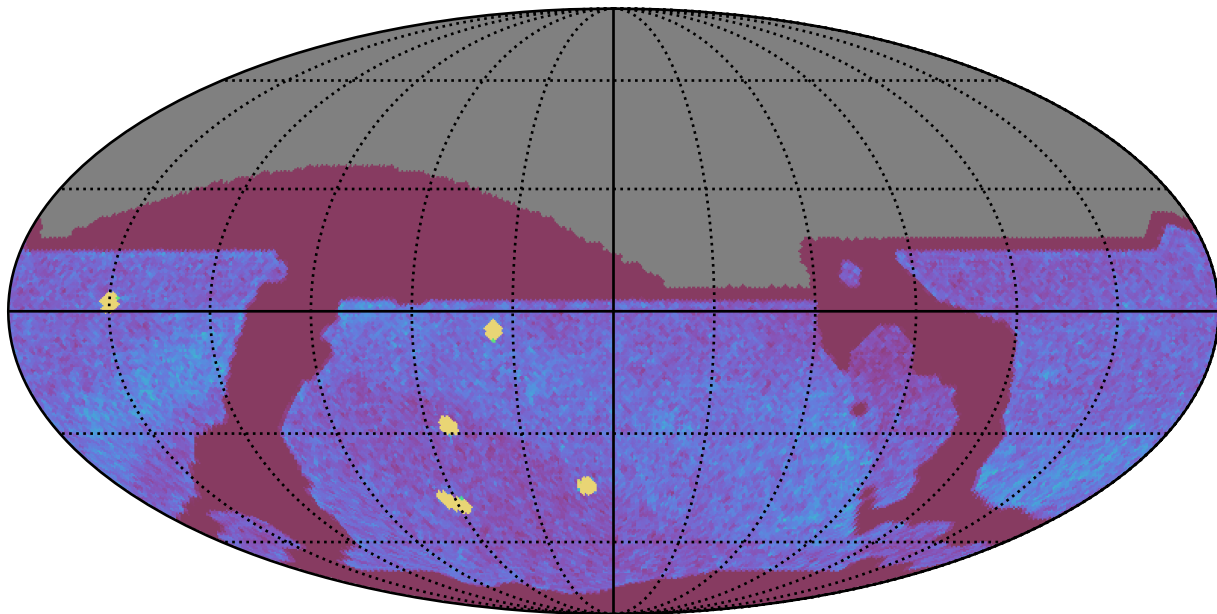
noroll_mjdp0_v3.4_10yrs All sky all bands: NVisits
