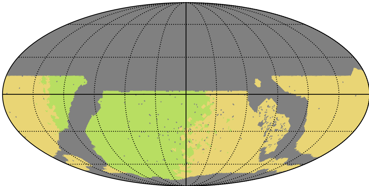
noroll_mjdp0_v3.4_10yrs WFD all bands: NSeasons
