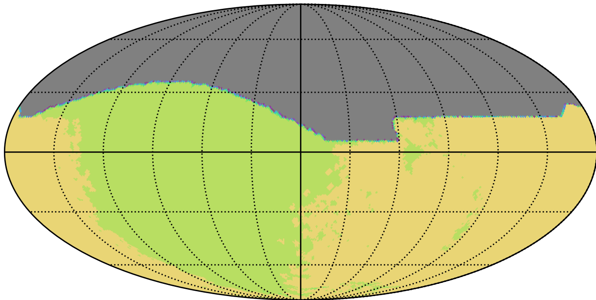
noroll_mjdp0_v3.4_10yrs All sky all bands: NSeasons
