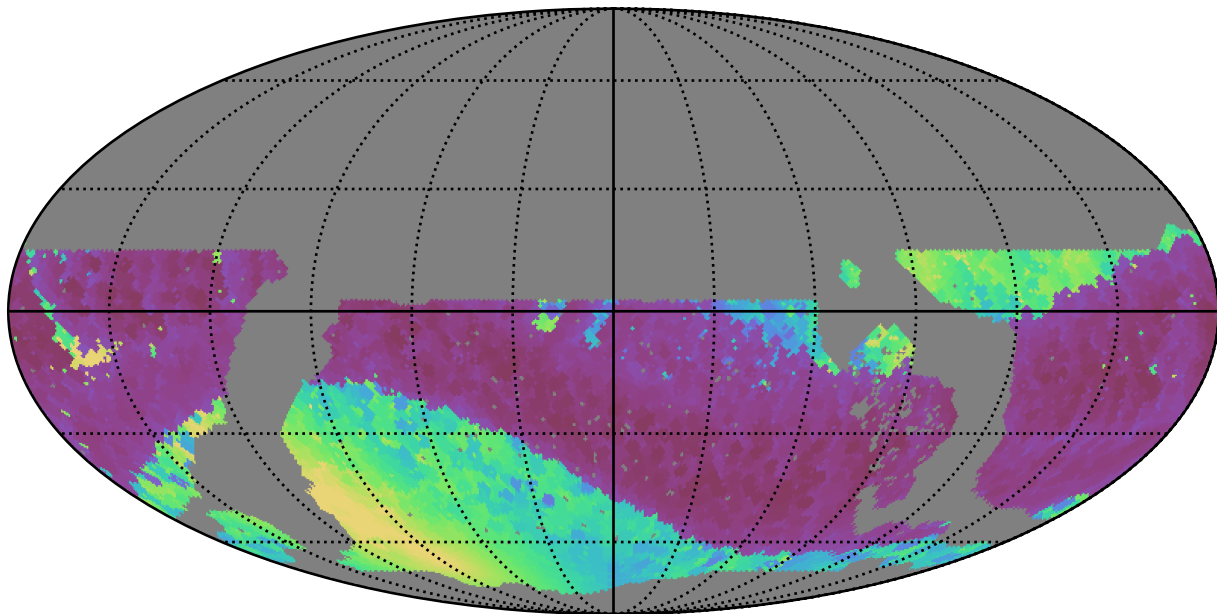
noroll_mjdp0_v3.4_10yrs WFD z band: Min solarElong
