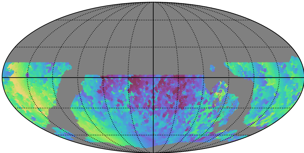
noroll_mjdp0_v3.4_10yrs WFD y band: Min solarElong
