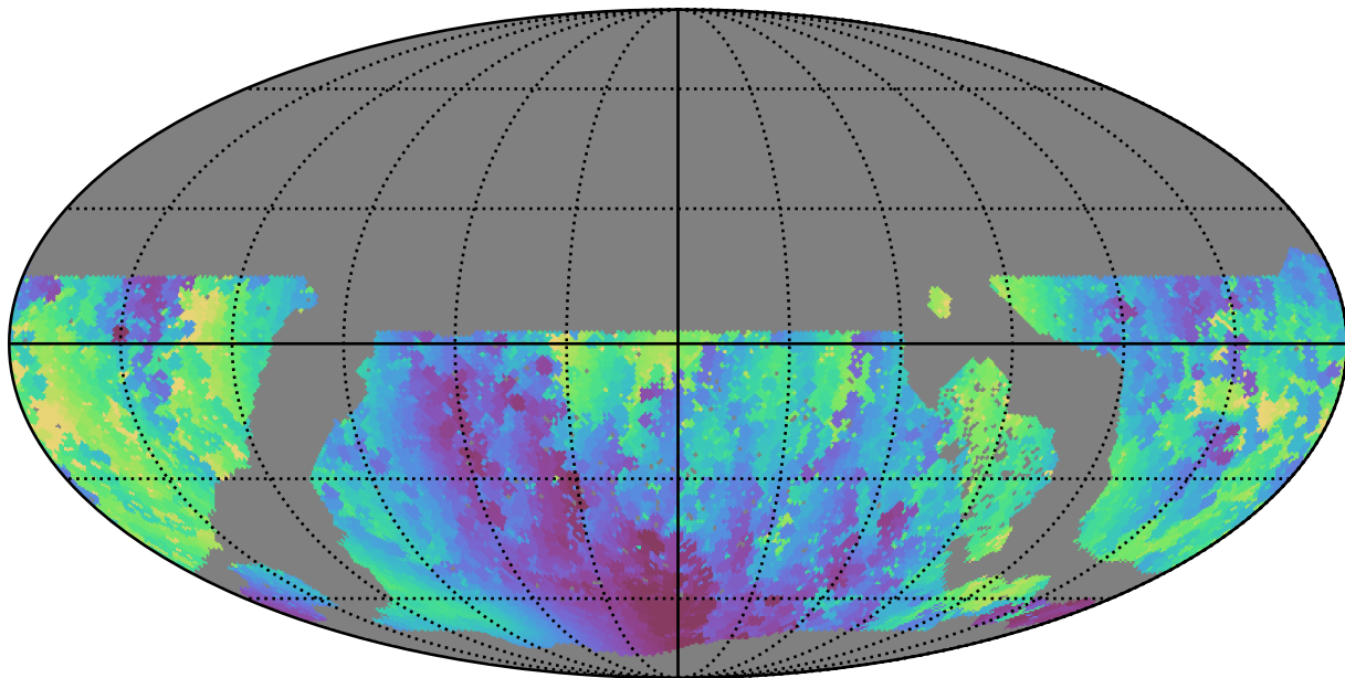
noroll_mjdp0_v3.4_10yrs WFD u band: Min solarElong
