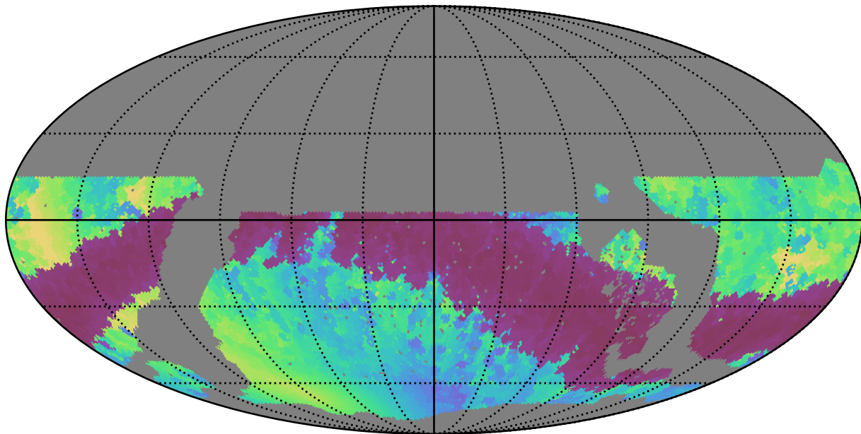
noroll_mjdp0_v3.4_10yrs WFD r band: Min solarElong
