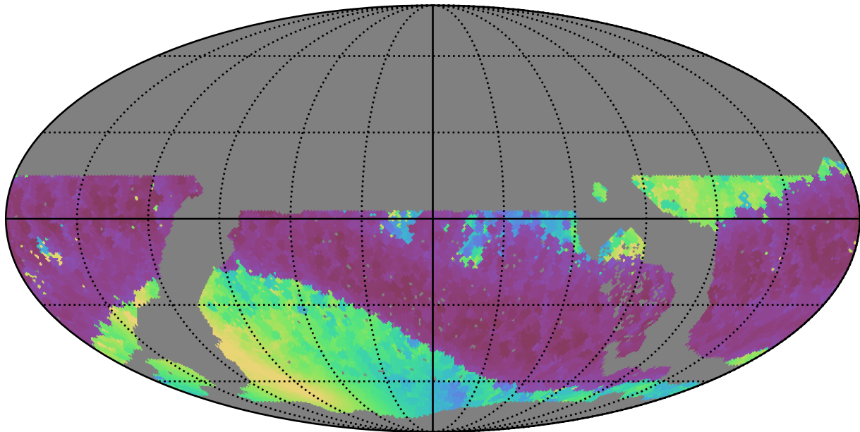
noroll_mjdp0_v3.4_10yrs WFD i band: Min solarElong
