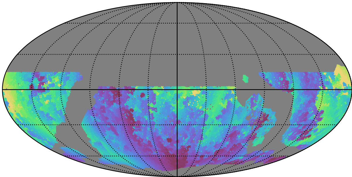
noroll_mjdp0_v3.4_10yrs WFD g band: Min solarElong
