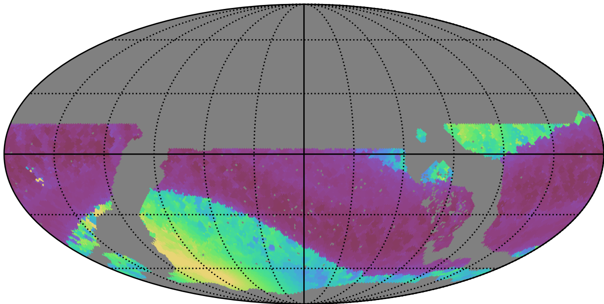
noroll_mjdp0_v3.4_10yrs WFD all bands: Min solarElong
