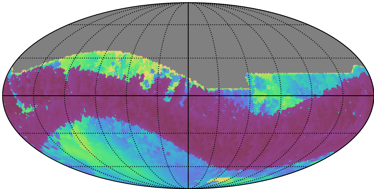
noroll_mjdp0_v3.4_10yrs All sky z band: Min solarElong
