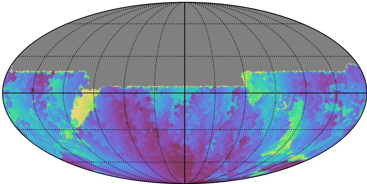
noroll_mjdp0_v3.4_10yrs All sky u band: Min solarElong
